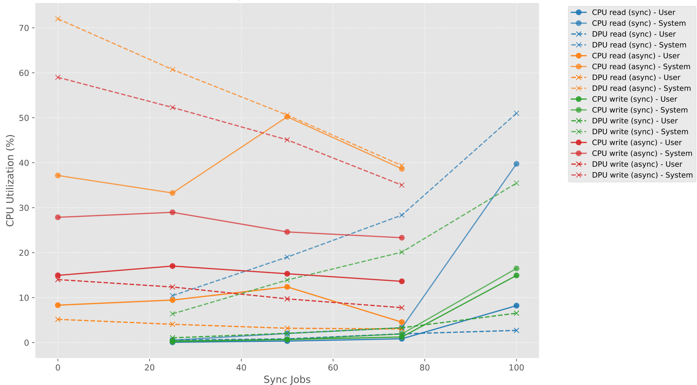
CPU Utilization vs Sync Jobs (mixed) - SEQ (CPU vs DPU)
